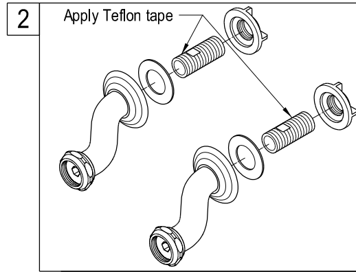
2. Apply Teflon tape on the threads of the copper shank. Install the elbow.
