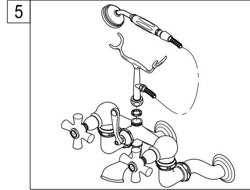
5. Place a washer between the side hole of the shower cradle and the cone nut of the shower hose. Tighten the cone nut.
