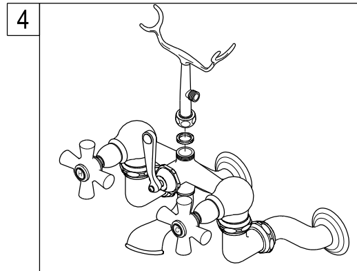
4. Install the shower cradle and spout on top of faucet body.
