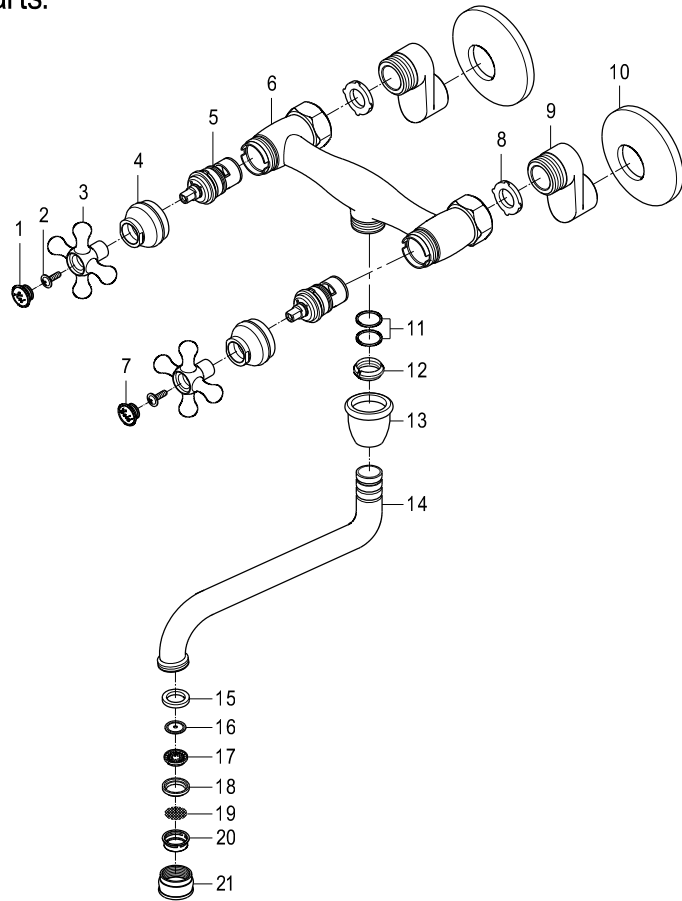
Cold Handle: KSH213C
