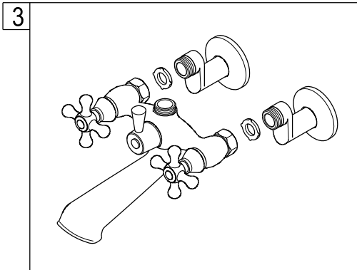
3. Apply Teflon tape on the threads of the elbow. Install the faucet.
